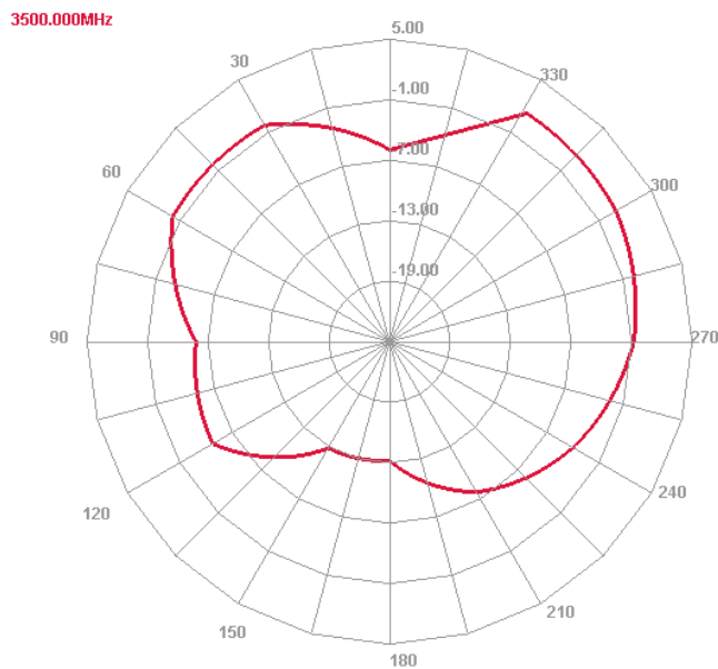
3500MHz H Plane
