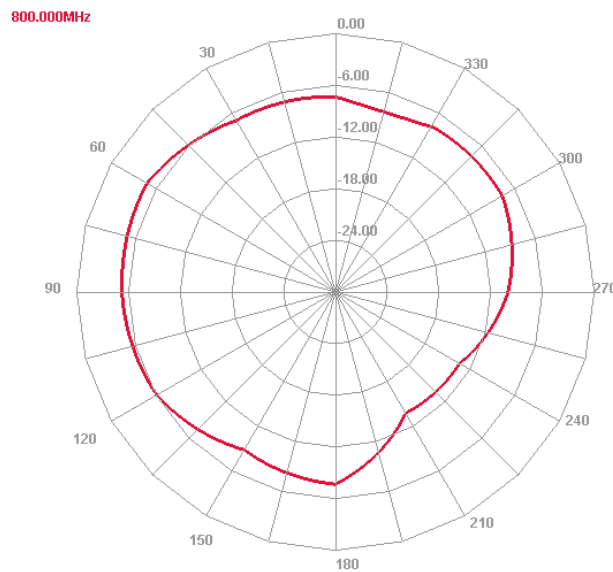
800MHz E Plane
