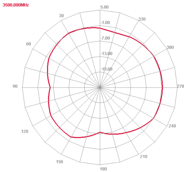
3500MHz E Plane
