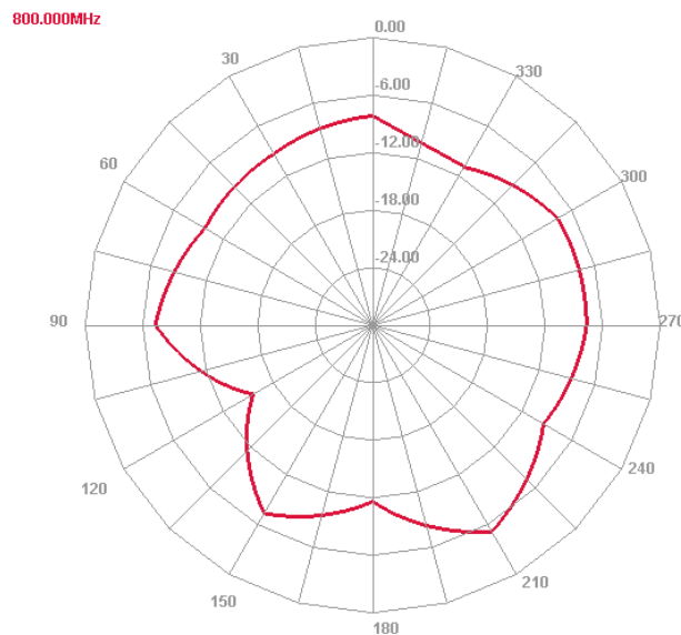
800MHz H Plane
