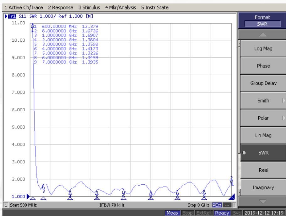
Measured VSWR
