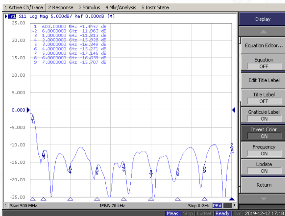
Measured S11
